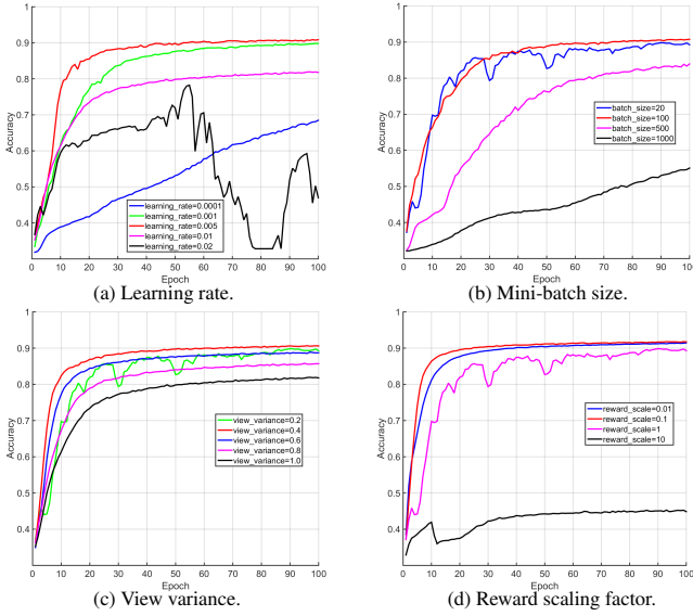
Figure 9: Evaluating four key hyper-parameters used in training MV-RNN. For each hyper-parameter, difference values are evaluated by plotting the recognition accuracy over epoch.
