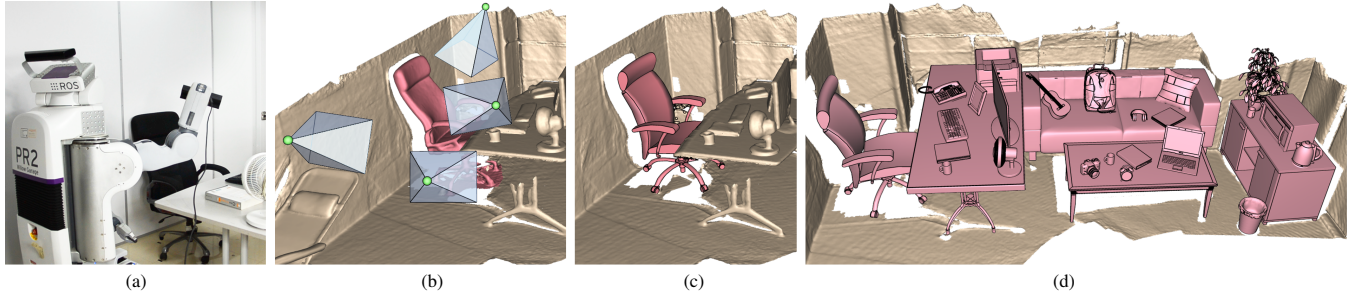
Figure 1: We present an autonomous system for active object identification in an indoor scene (a), with consecutive depth acquisitions. The scene is first roughly scanned, and segmented to generate 3D object proposals. Targeting an object proposal (b), the robot performs multi-view object identification, based on a 3D shape database, driven by a 3D Attention Model. The retrieved 3D models are inserted into the scanned scene (c), replacing the corresponding object scans, thus incrementally constructing a 3D scene model (d).
