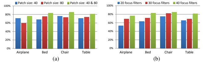
Figure 13: Accuracy of fine-grained classification on four datasets with varying patch sizes (a) and focus filter counts (b). The classification is performed on single-view images with partial occlusion.
